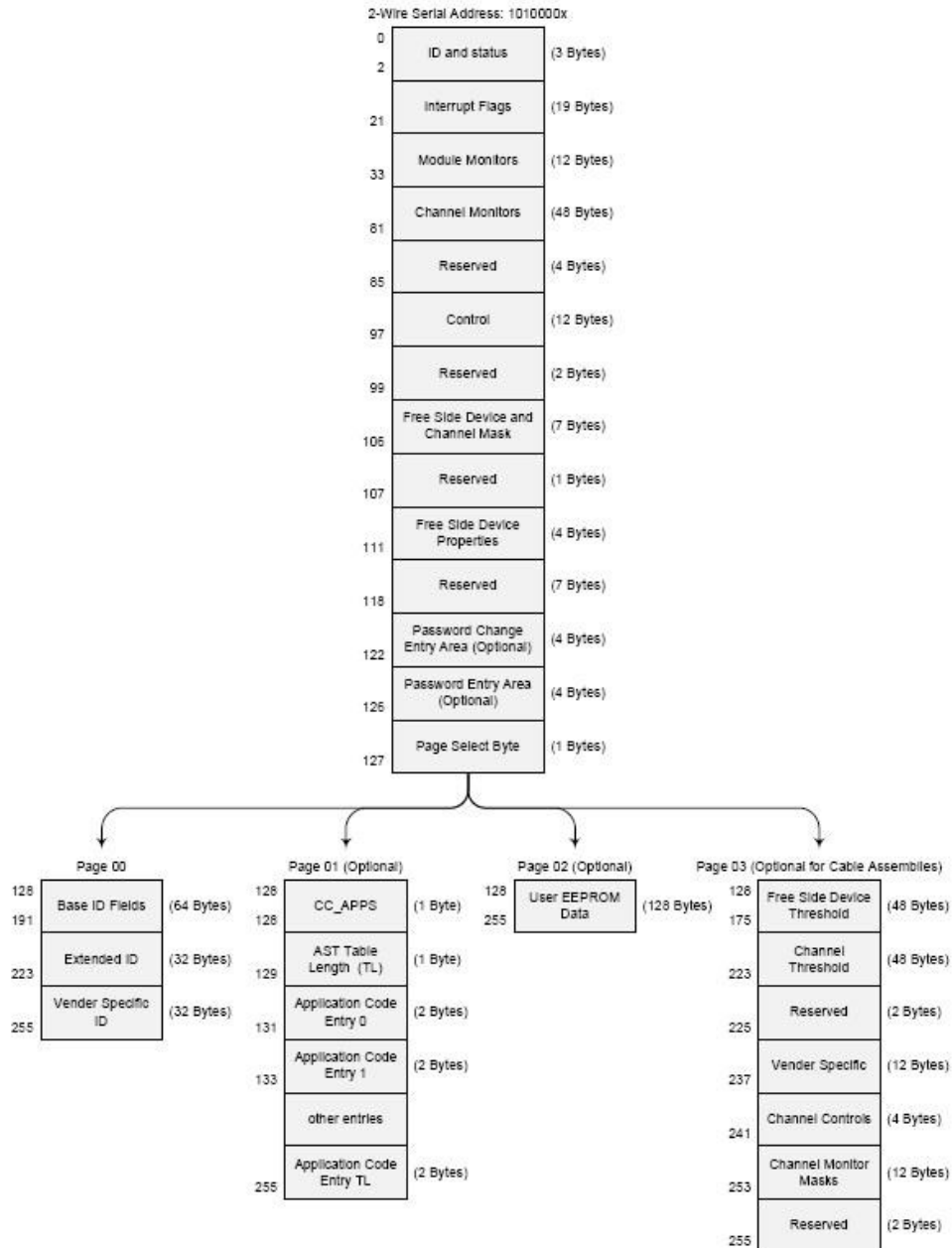
Figure5.QSFP Memory Map
