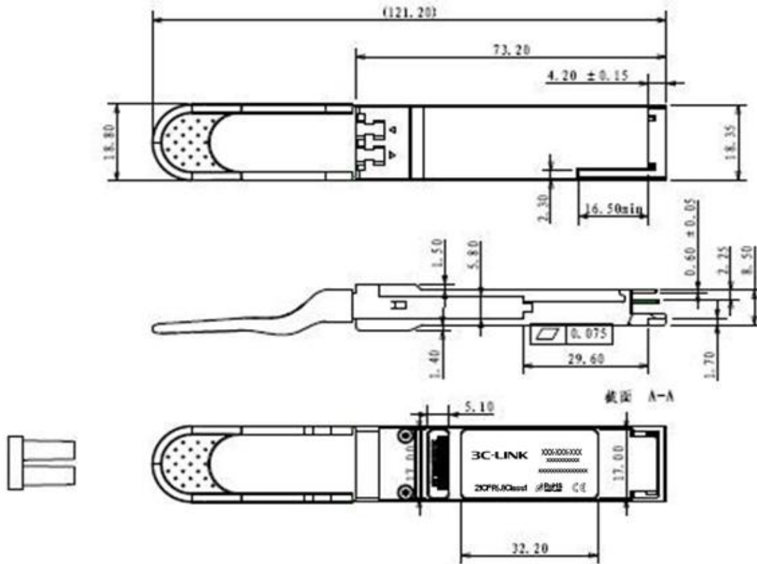
Figure10.Mechanical Specifications
