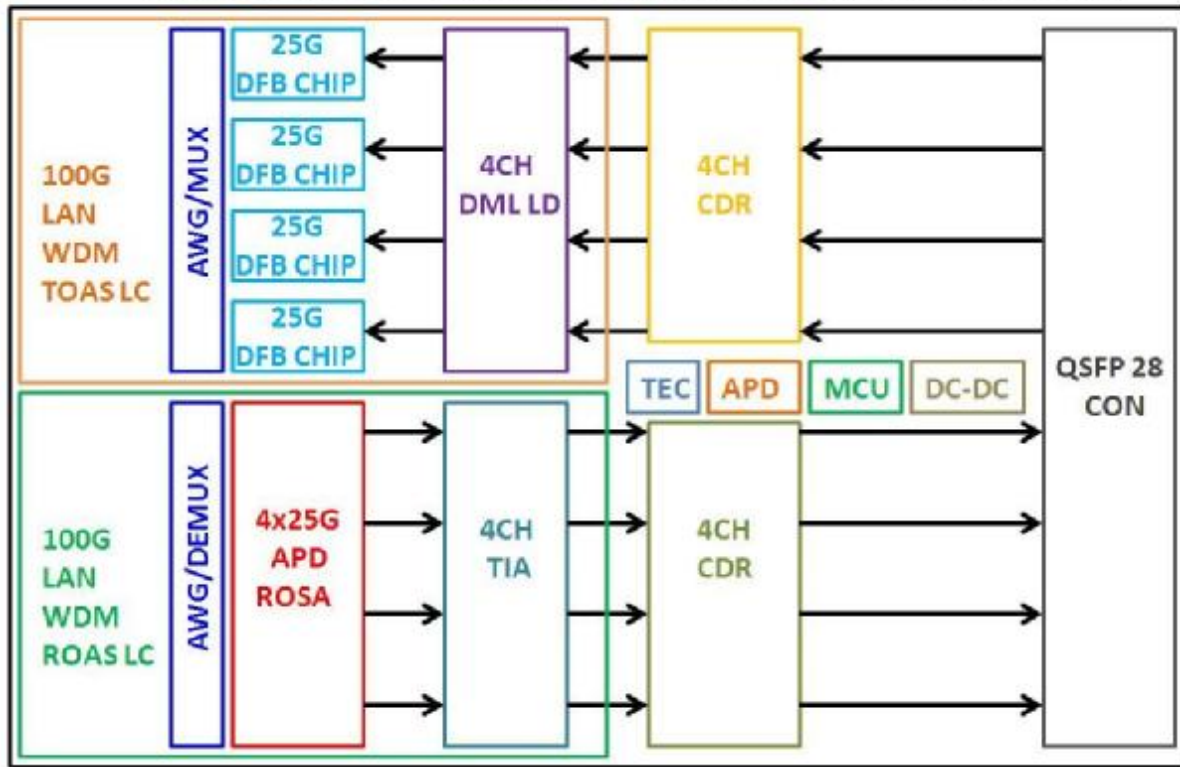
Figure1.Module Block Diagram
